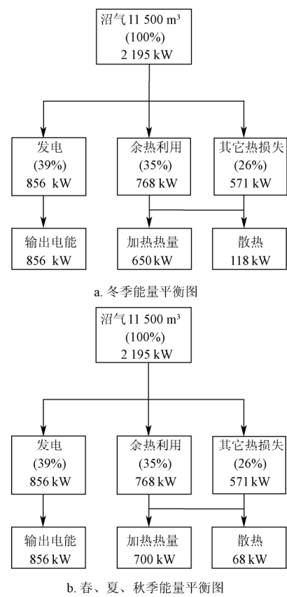
图 6 蒙牛澳亚示范牧场沼气工程全年能量平衡图 Fig.6 Energy balance of biogas engineering at Mengniu-Macao Demonstration Pasture
